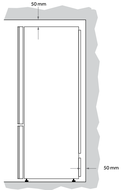
Installation distance
